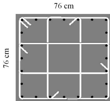
Fig. 1. Column cross-section
