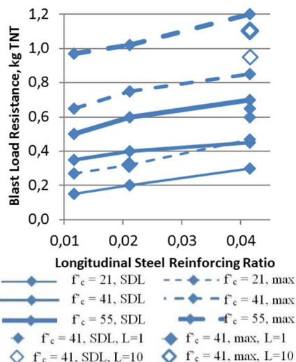
Fig. 4. Effect of reinforcement ratio
